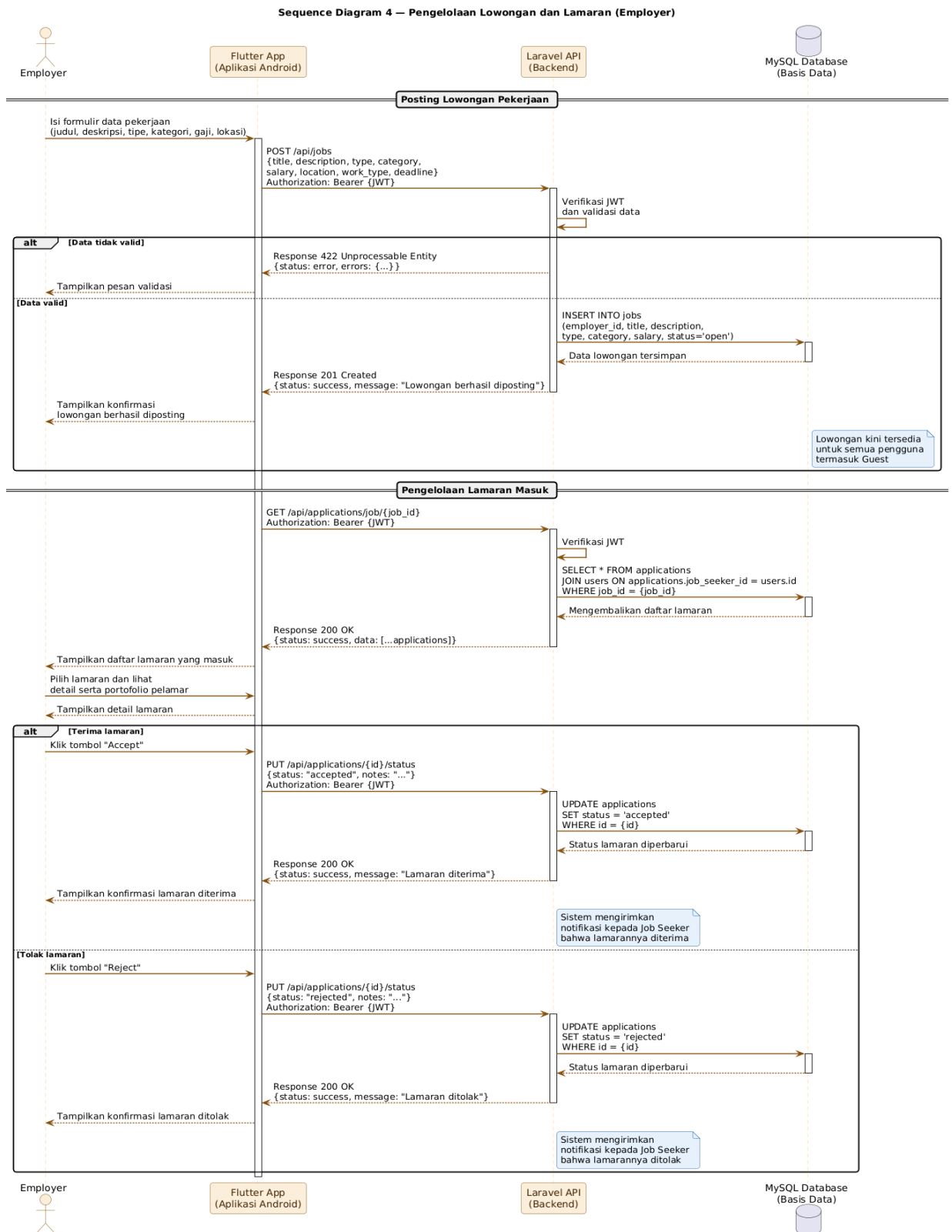
gambar 11.sequence diagram pengelolaan lamaran
