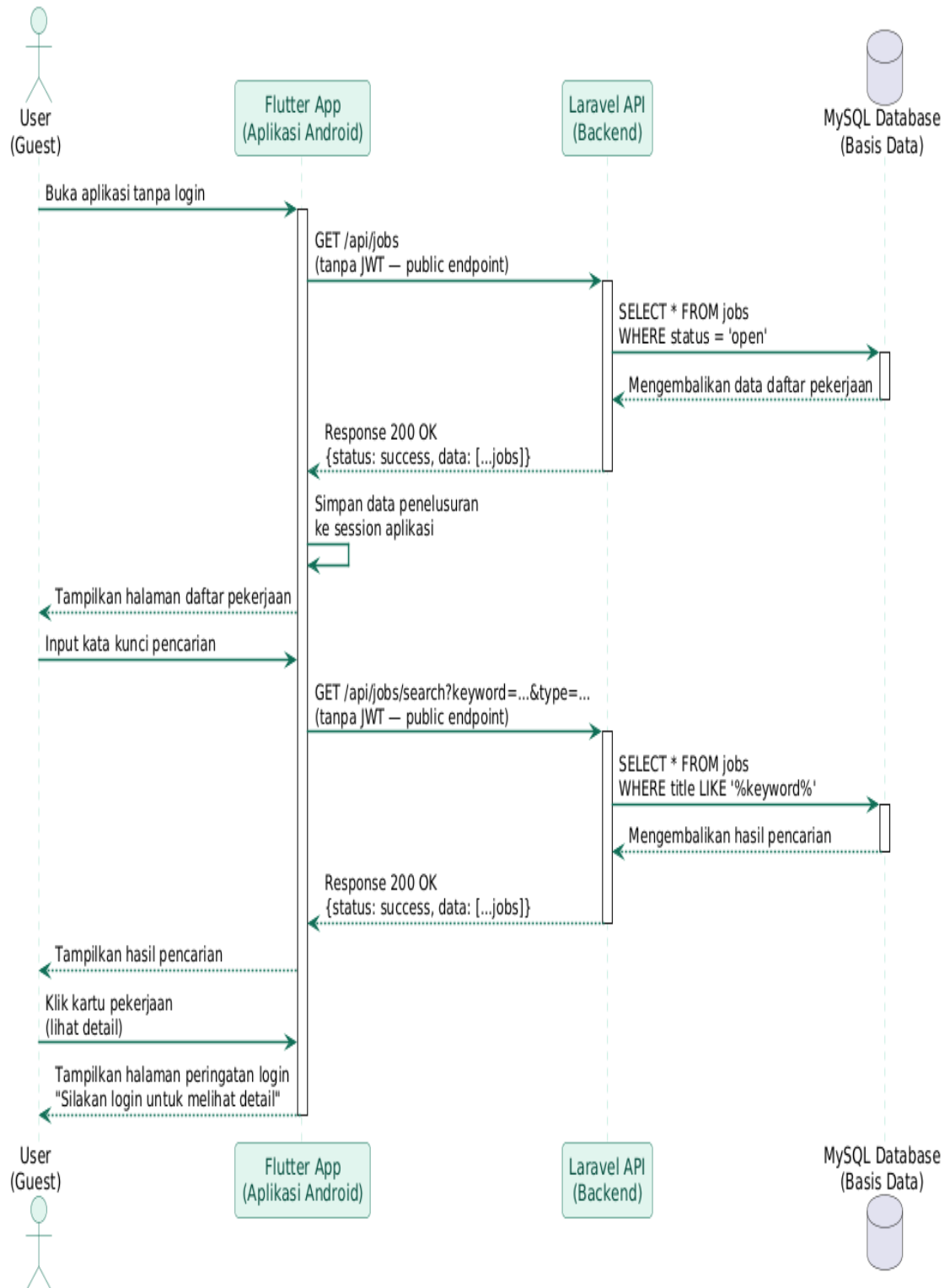
Sequence Diagram 1 – Guest Mode
