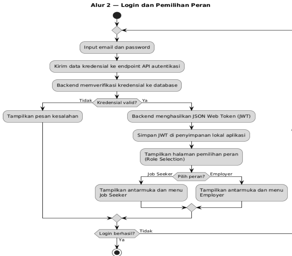
gambar 4. Activity diagram login
