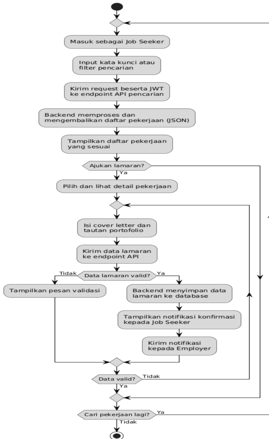
gambar 5. Activity diagram pencarian pekerjaan
