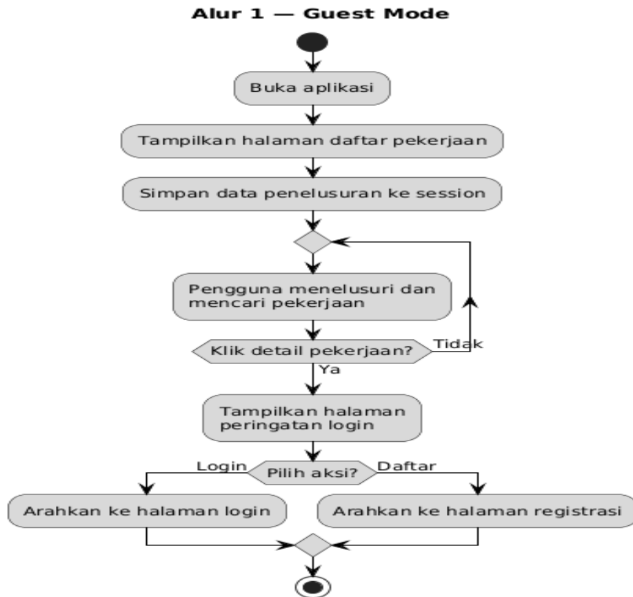
gambar 3.activity diagram guest mode
